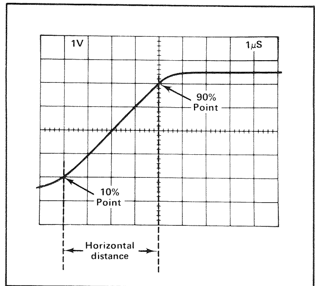
Fig. 1-14. Measuring risetime.
